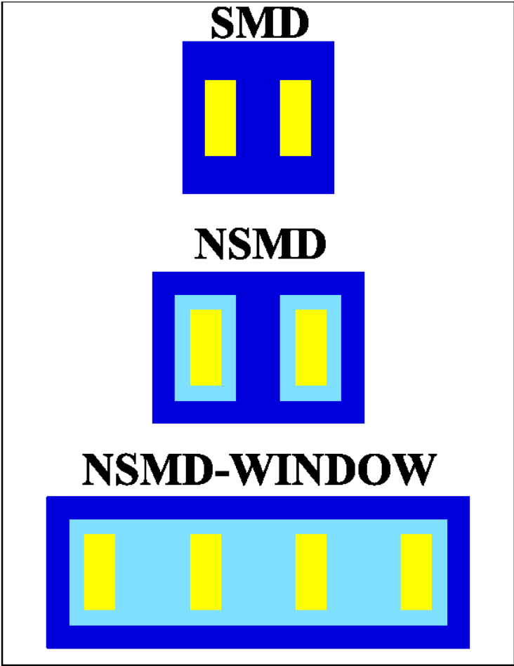
Figure 3 Solder Mask Designs
