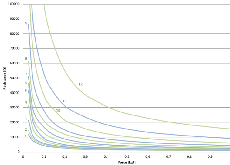
Figure 10: Examples of force sensitive profiles, resistance as a function of force, for various material blends
