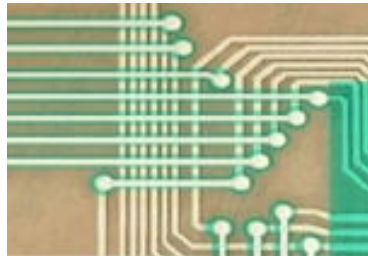
Figure 8: An example of a multi-layered print with dielectric crossover
