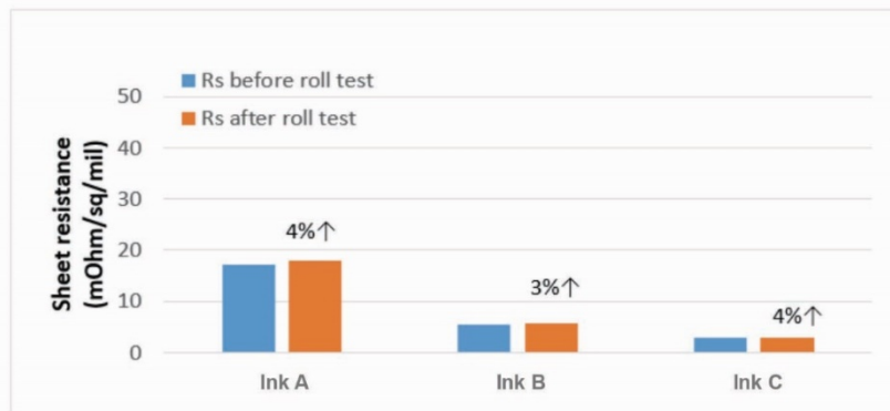
Figure 5: Sheet resistance of silver conductive inks before and after roll test
