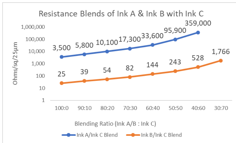
Figure 9: Sheet resistance ranges of blended FSR ink systems
