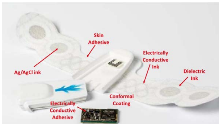
Figure 7: Typical sensor pad on flexible substrate representing a multiple layer build
