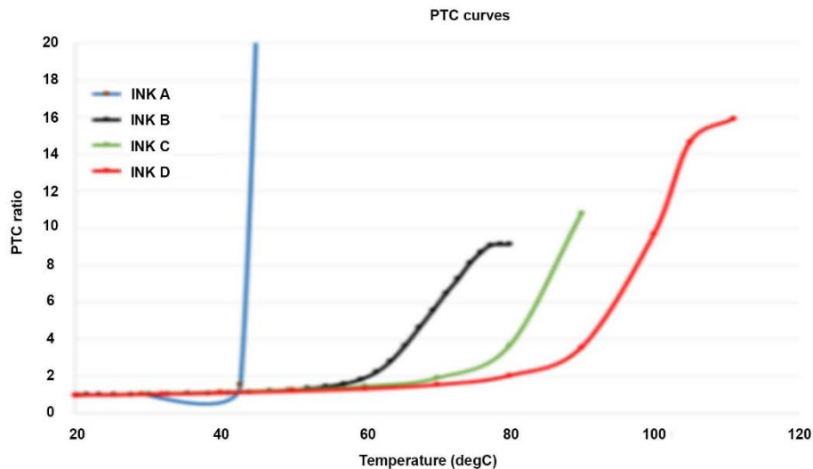
Figure 12: Plot of PTC ink maximum temperature curves
