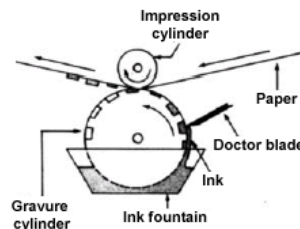
Figure 2: A typical rotogravure type system
