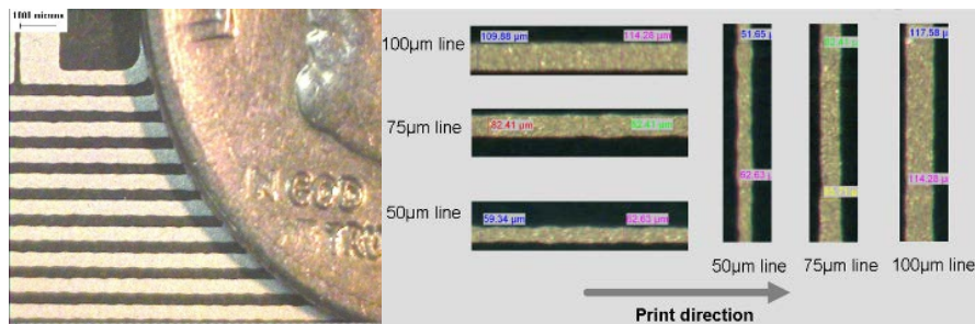
Figure 4: Typical conductive traces for fine line printing capabilities
