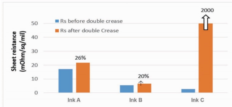
Figure 6: Sheet resistance before and after double crease test
