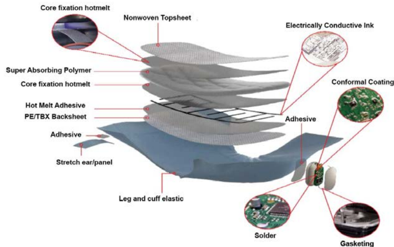
Figure 11: Example of a smart diaper designed for moisture sensing and monitoring
