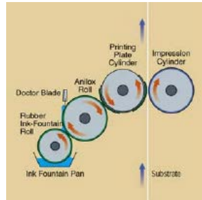
Figure 1: A typical flexographic press design
