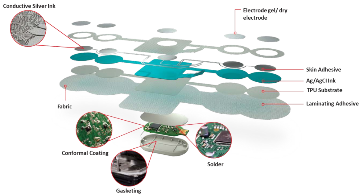
Figure 112: Example of a smart patch build utilizing Ag and AgCl inks
