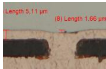
Figure 10 - Achieved Cu Thickness distribution on a 600\times 600\text{mm} Panel
