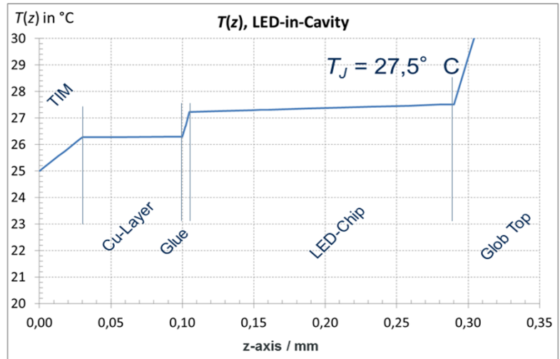
Figure 13. Results: Temperature profile along the symmetry axis in out-of-plane direction ( z -axis) of a LED-in-Cavity set-up
