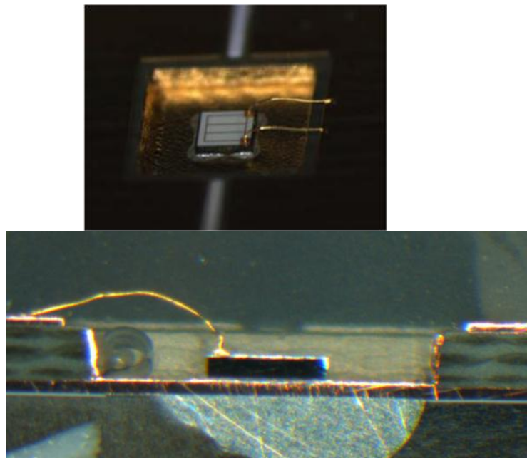
Figure 8. Chip in cavity bonded to the upper layer
