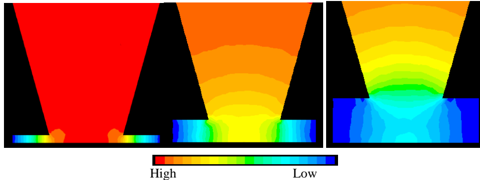
Figure 3. Pressure drop vs. different dispensing height. (a) 5 microns. (b) 15 microns. (c) 30 microns.
