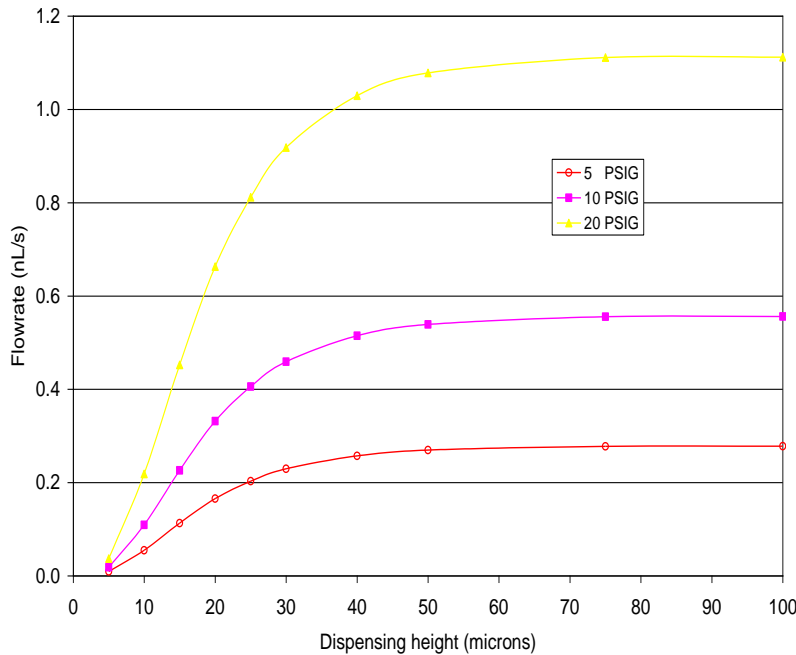
Figure 4. Flow Rate versus Dispense Height
