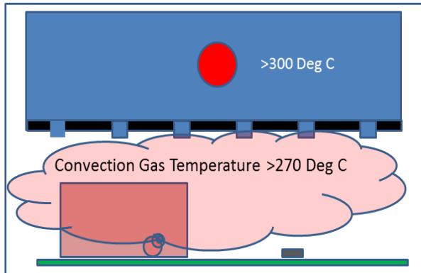
Figure 3. Convection soldering - Excessive source temperature can affect low mass parts
