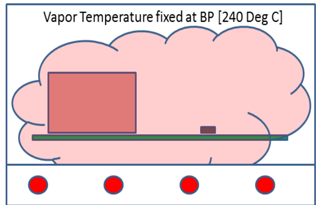
Figure 1. Vapor Phase Fluid BP determines peak temperatures for ALL components.
