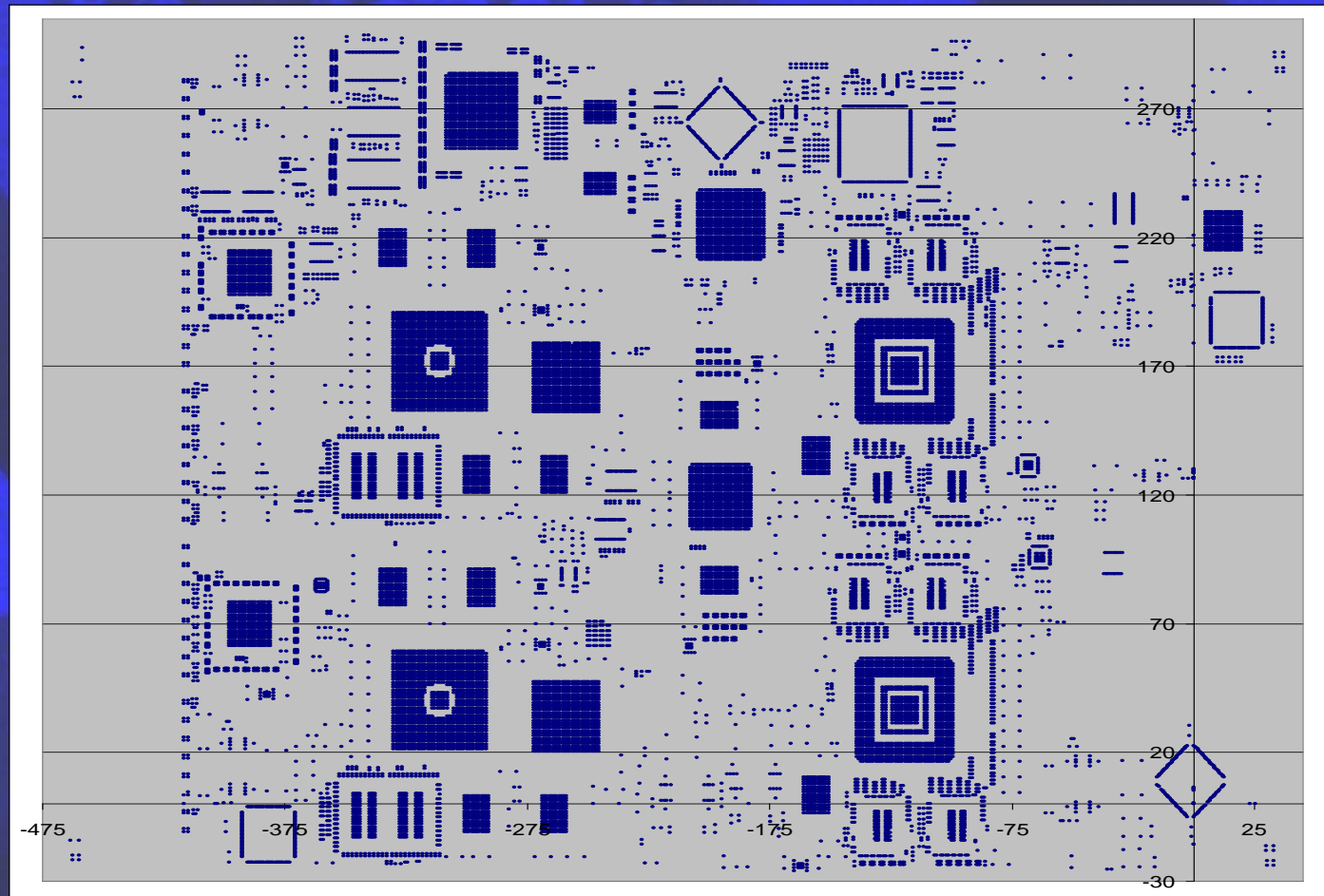
21,000 apertures, 350x500mm
