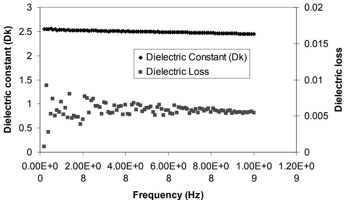
Figure 9: Dielectric constant and loss as a function of frequency for epoxy filled system.
