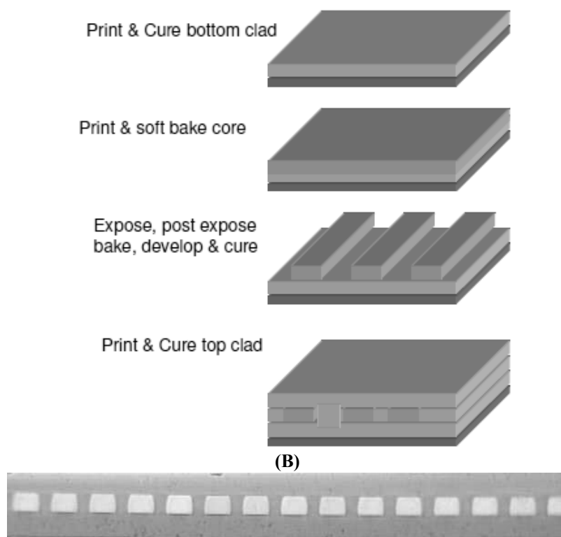
Figure 8: (A) Schematic presentation for making printable waveguides and (B) optical waveguides.
