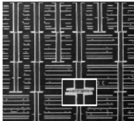
Figure7 : Photograph of z-interconnect laminate shown in cross section.
