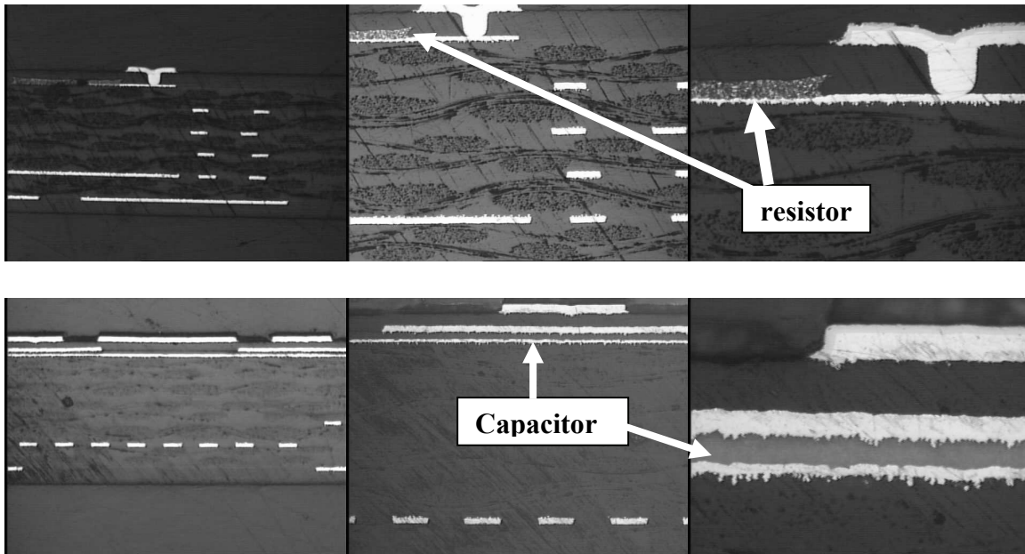
Figure 5A: Cross-section view of screen printed embedded capacitors and resistors.
