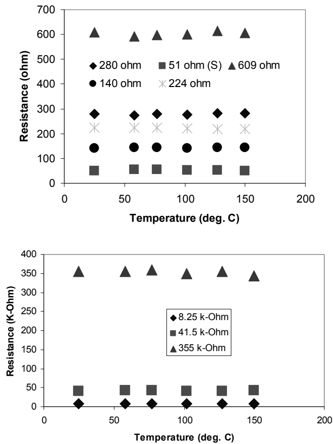
Figure 6: Change in resistance with Temperature.
