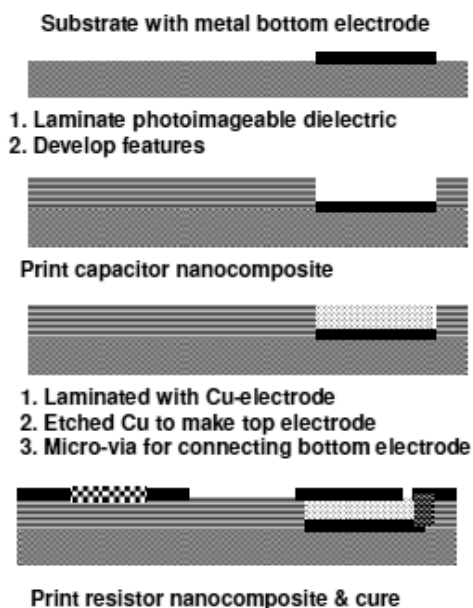
Figure 4: Schematic presentation for making screen printable thin film embedded capacitors and resistors.
