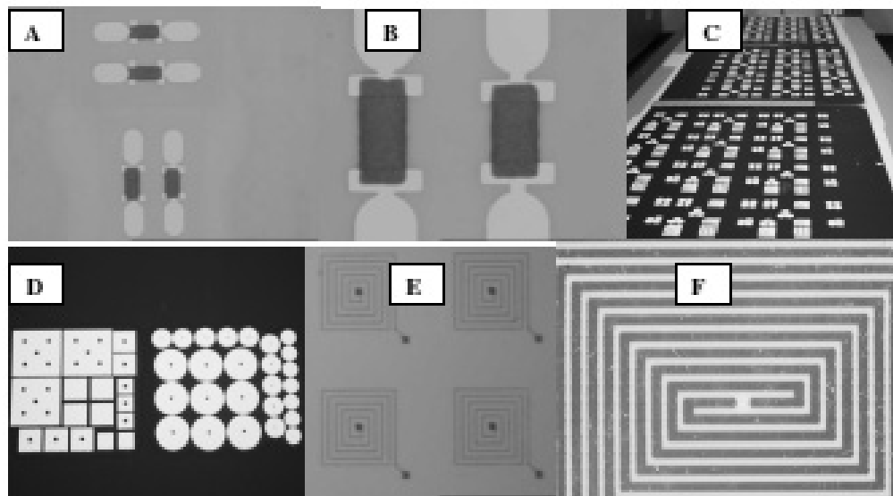
Figure 2: Various printing process (A)-(B) screen printed resistors, (C)-(D) screen printed capacitors, and (E)-(F) Ink-jet printed inductors.
