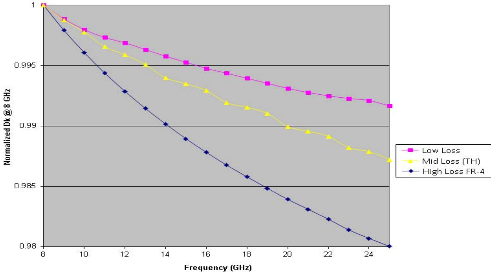
16mil Balanced Stripline Transmission Line, Differential Phase Length Method
