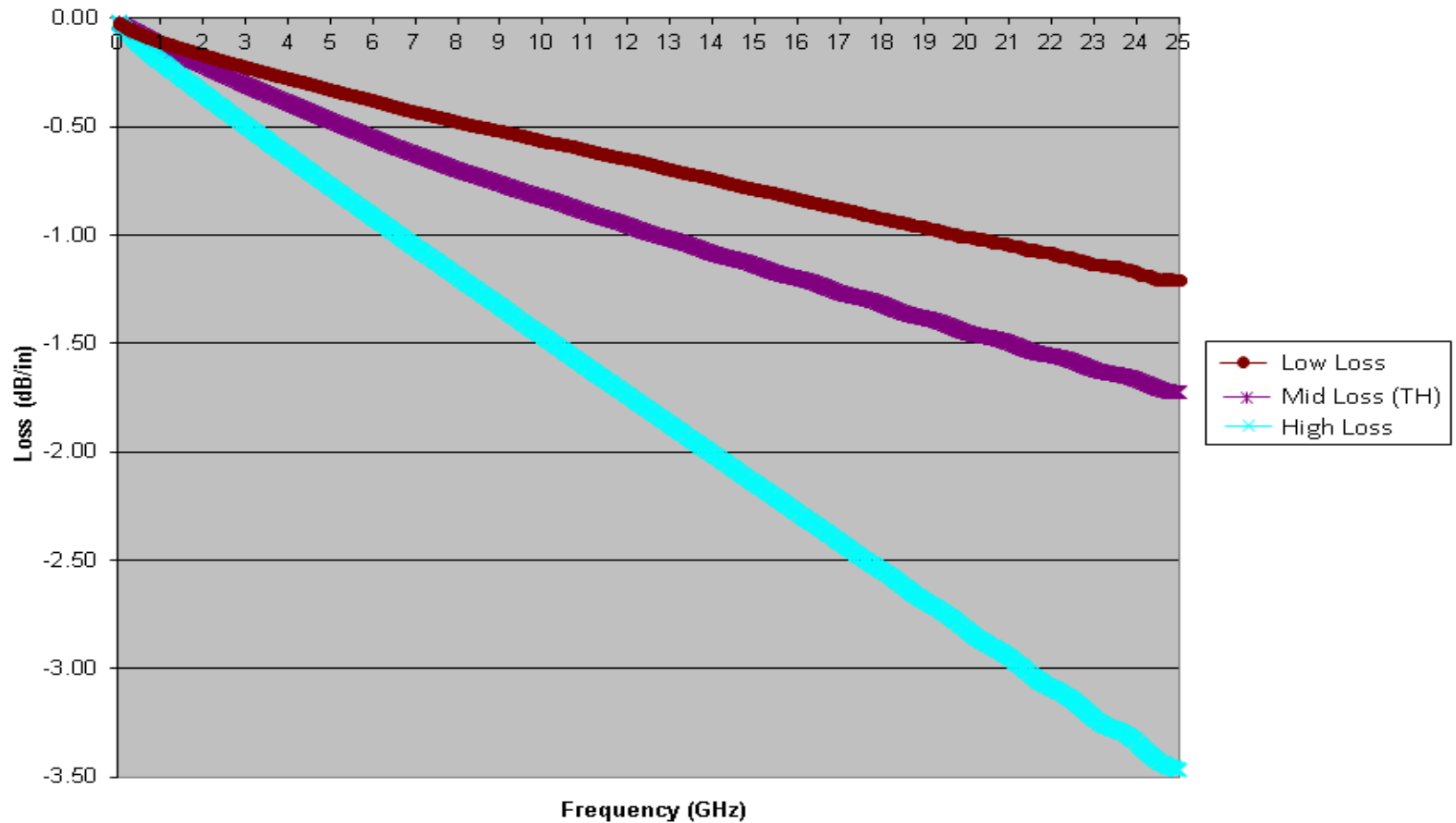
16mil Stripline Transmission Line Circuits, Insertion Loss, Differential Length Method
