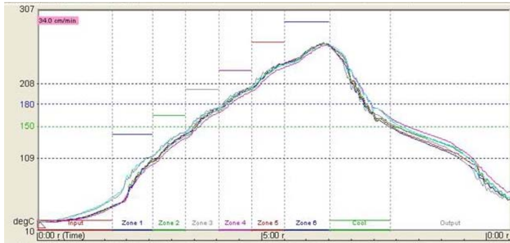
Figure 3. Typical lead-free soldering reflow cycle.
