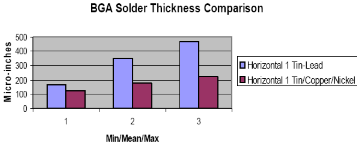
Figure 16. Comparison of HASL coating thickness (Fellman 7 )
