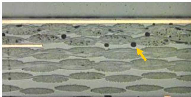
Figure 2. Voids in laminate resin due to excessive exposure to heat
