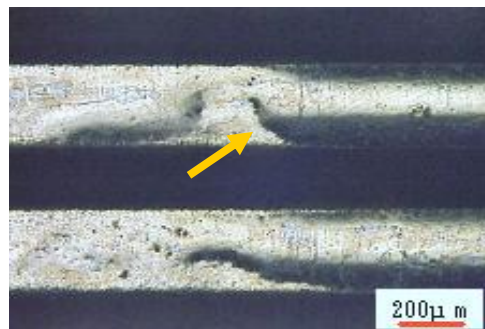
Figure 9. Dewetting of the solder coating
