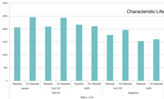
Figure 8. Characteristic Life: PBGA1156 – FR4-06 – No Aging
